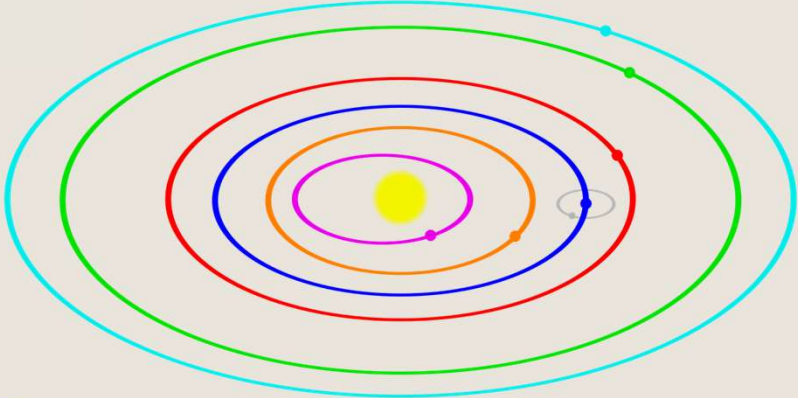
Kepler/Newton
